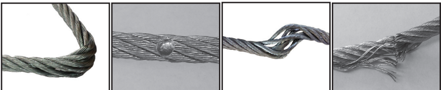
IMAGE 1: CABLE DAMAGE EXAMPLES
