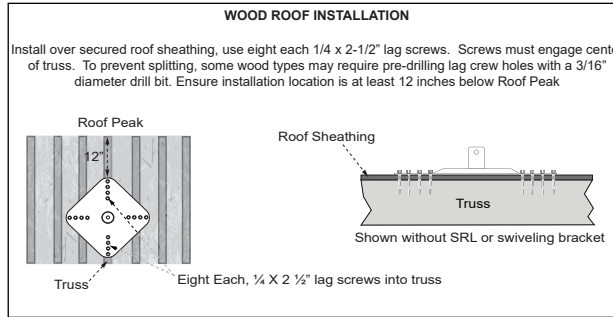
FIGURE 9 - INSTALLATION
