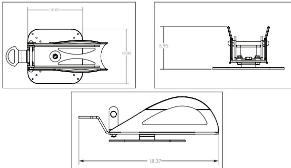
FIGURE 6 - DIMENSIONS (In Inches)
