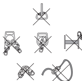
FIGURE 3 - INAPPROPRIATE CONNECTIONS
