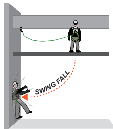
FIGURE 1 - SWING FALLS
