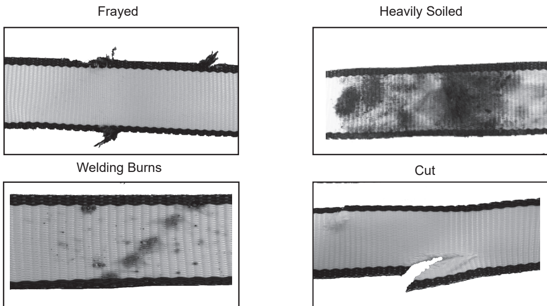
FIGURE 9 - EXAMPLES OF EQUIPMENT DAMAGE Webbing Damage Examples
